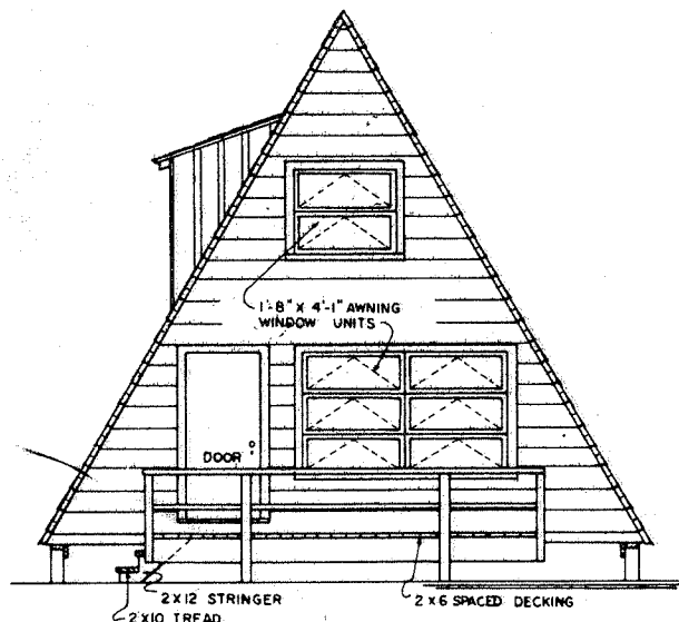
DECK-END ELEVATION
