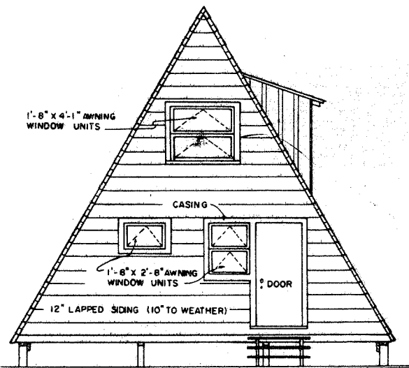
REAR ELEVATION
